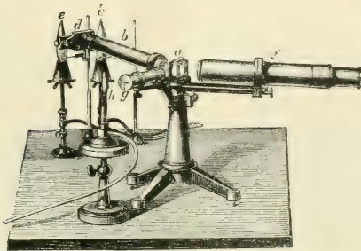
FIG. 5.—Observation of a flame spectrum with ordinary spectroscope with comparison prism. a , prism; b , collimator; d , slit; e e' , flames to be compared; f , observing telescope; g , scale illuminated by h and reflected by the second surface of the prism into the telescope.
